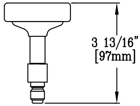
T&S NO. EB-1421 REGULAR SPRAY QUICK CONNECT
