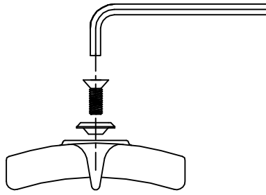
VANDAL PROOF KIT USED WITH T&S 4-ARM HANDLES
